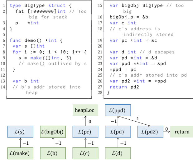
Figure 1. Go code and its escape graph. The escape graph determines whether a location (a node in the graph) is allocated on the stack (blue) or heap (green) by solving memory constraints. Virtual locations (nodes without frames: heapLoc and return ) are dummy nodes for simplifying analysis. Numbers on edges are explained in table 2.
