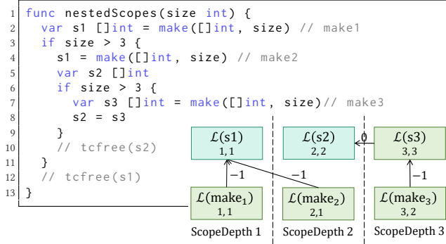
Figure 6. Nested scopes. Numbers under each node are their DeclDepth() and OutermostRef() values.
