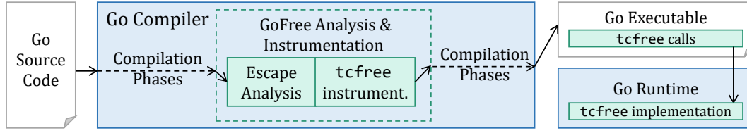
Figure 2. Architecture of GoFree. Blocks in blue are existing components of the Go compiler and runtime. Blocks in teal are new to GoFree. At compile time, GoFree inserts explicit deallocation ( tcfree calls) in the executable. At run time, tcfree calls into the enhanced Go runtime. The GoFree enhancements are fewer than 2000 lines of code in total.
