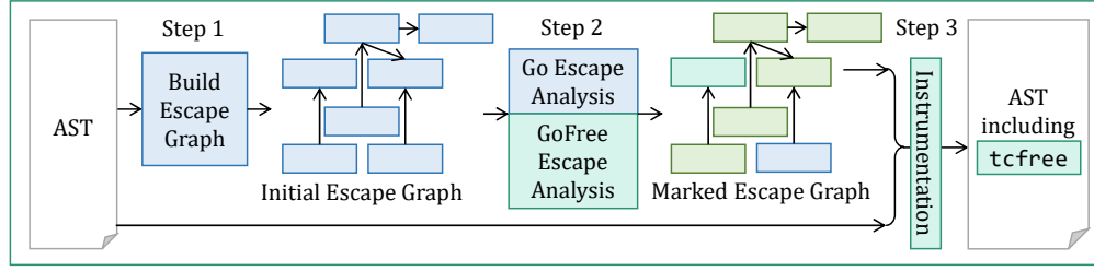
Figure 4. GoFree static analysis and instrumentation. GoFree reuses Go’s original escape graph, marking nodes with different properties (such as HeapAlloc ) after escape analysis to meet both Go’s and GoFree’s constraints. tcfree calls are then inserted into the AST according to these properties. Blue and green boxes are in the original Go system. Teal boxes are new to GoFree.
