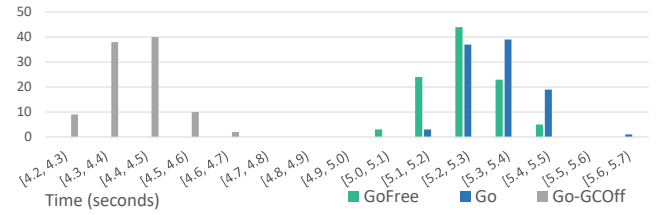
Figure 11. Run time distribution across 99 runs under each of the 3 settings respectively: original GoFree, original Go, and original Go with GC turned off.
